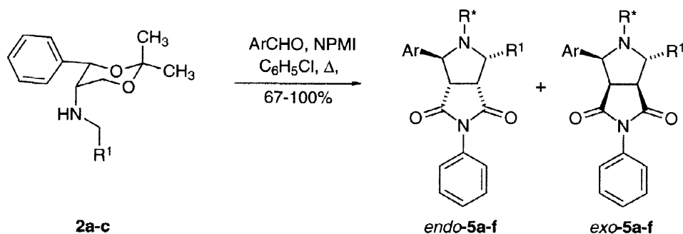
Scheme 2. Diastereoselective cycloadditions utilising NPMI
