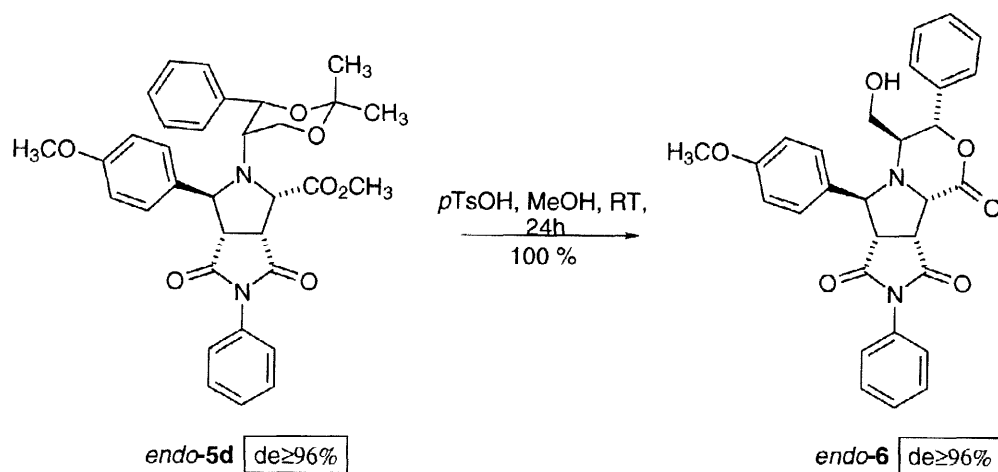
Scheme 3. Chemoselective intramolecular lactonization
