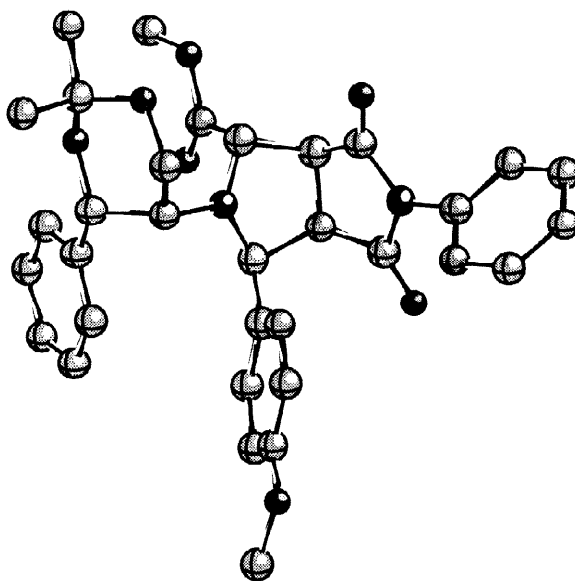
Figure 3. Structure of exo - 5d in the crystal
