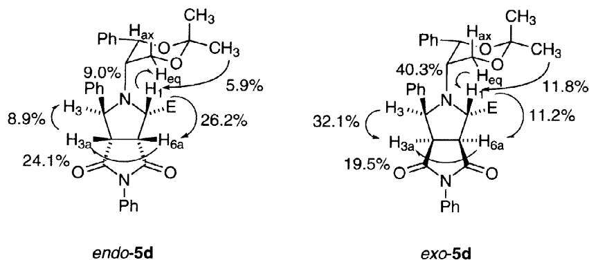
Figure 2. Observed NOE effects on 5d
