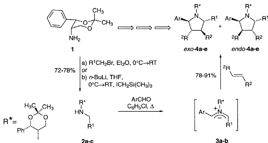
Scheme 1. Diastereoselective 1,3-dipolar cycloadditions
